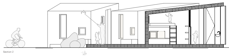
Section 2
