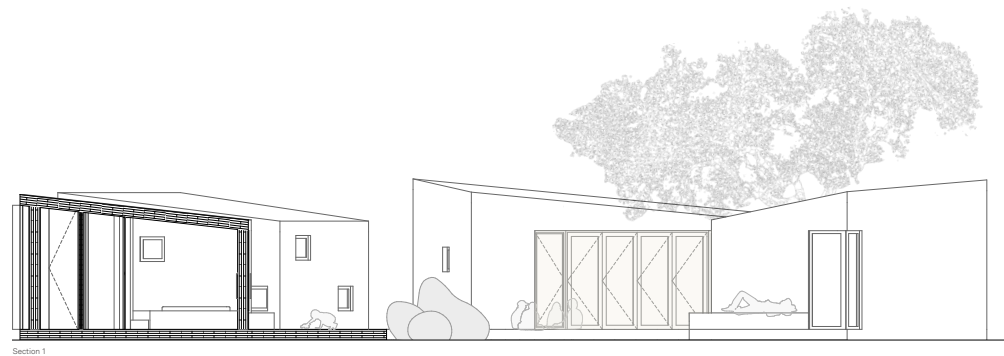
Section 1
